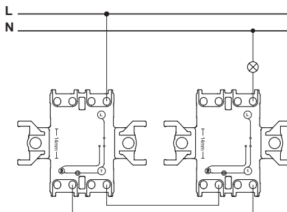
Two 2-way switches with locator lamps
