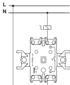
Push-button
