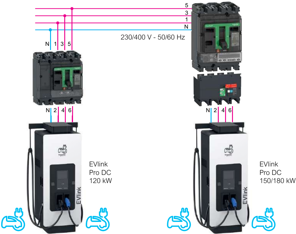
Current information and protections to use with EVlink Pro DC 120 - 150 - 180 kW
