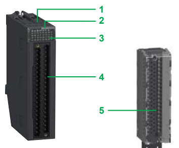
Module for connection via 40-way removable terminal block
