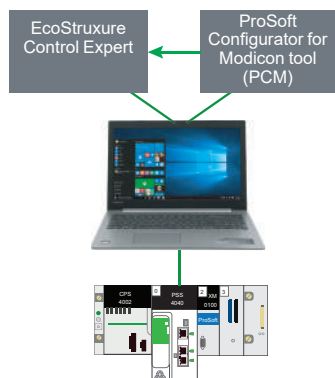
Interaction between EcoStruxure Control Expert, Prosoft Configurator for Modicon (PCM tool), and Modicon X80 PROFIBUS DP module
