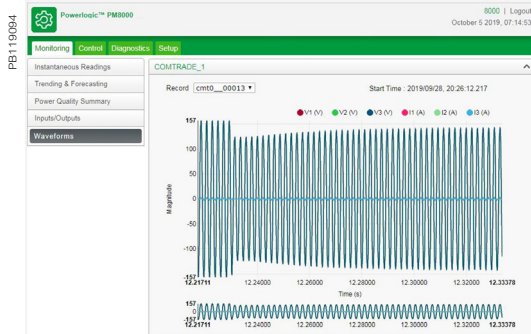
PowerLogic PM8000 series waveform web page sample
