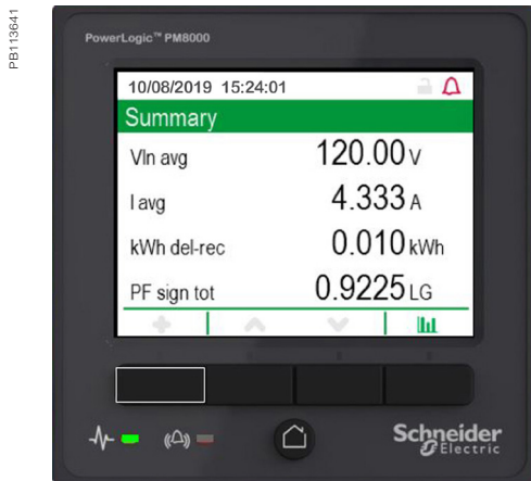
PowerLogic PM8000 series meter.
