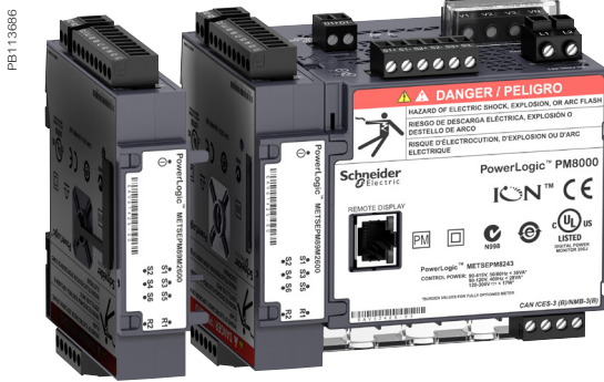
PowerLogic PM8000 series meter with I/O modules.
