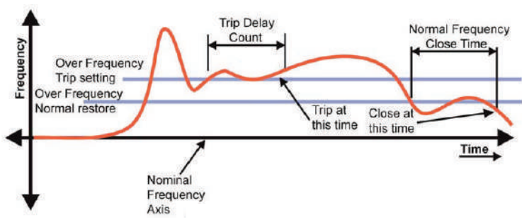
Under/over frequency protection
