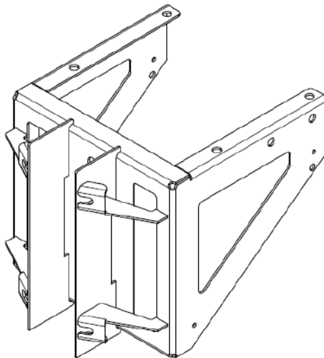
End mounting
