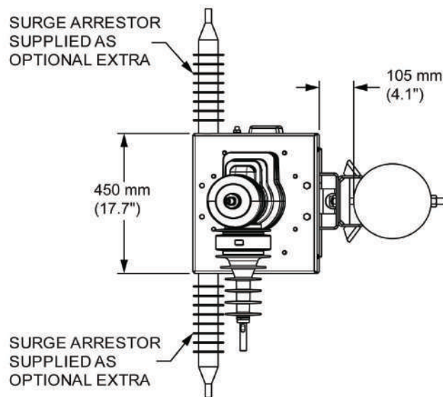
Overhead view of PMSet W-Series mounting arrangement
