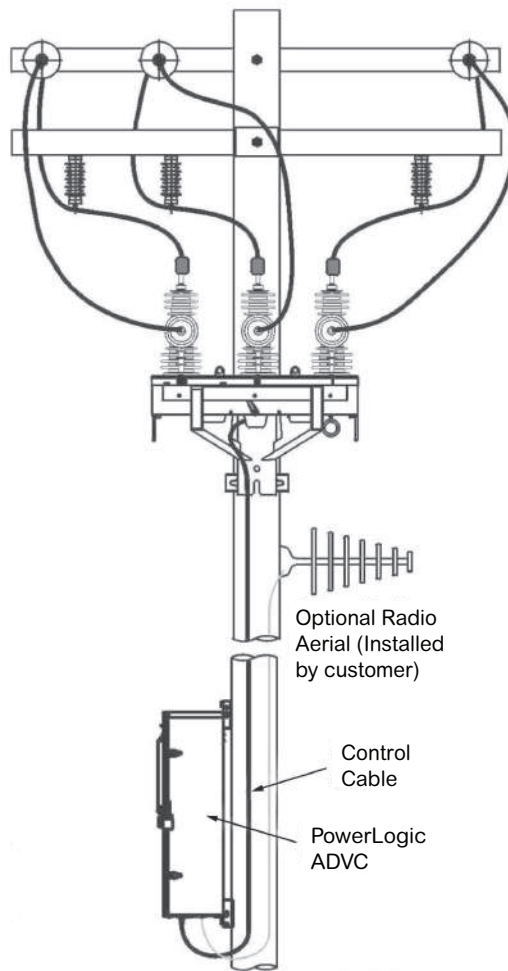
Pole mounted PMSet U-Series recloser with PowerLogic ADVC
