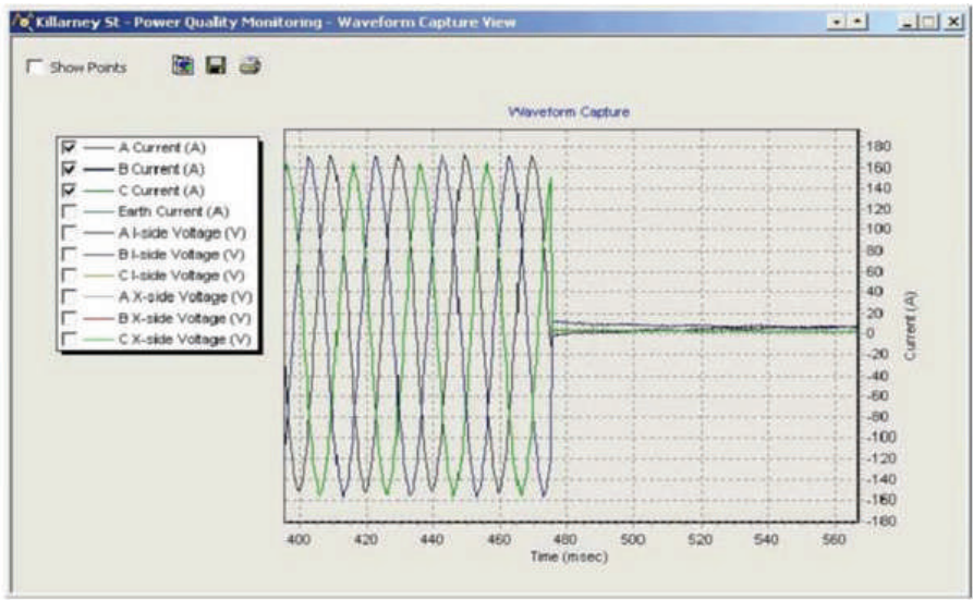
Waveform capture
