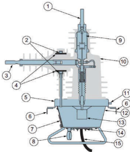
Cross section of PMSet U-Series
