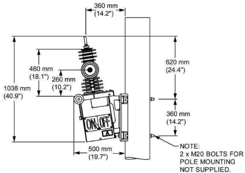
Side view of PMSet W-Series mounting arrangement
