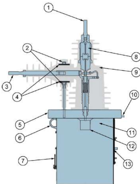
Cross section of PMSet W-Series
