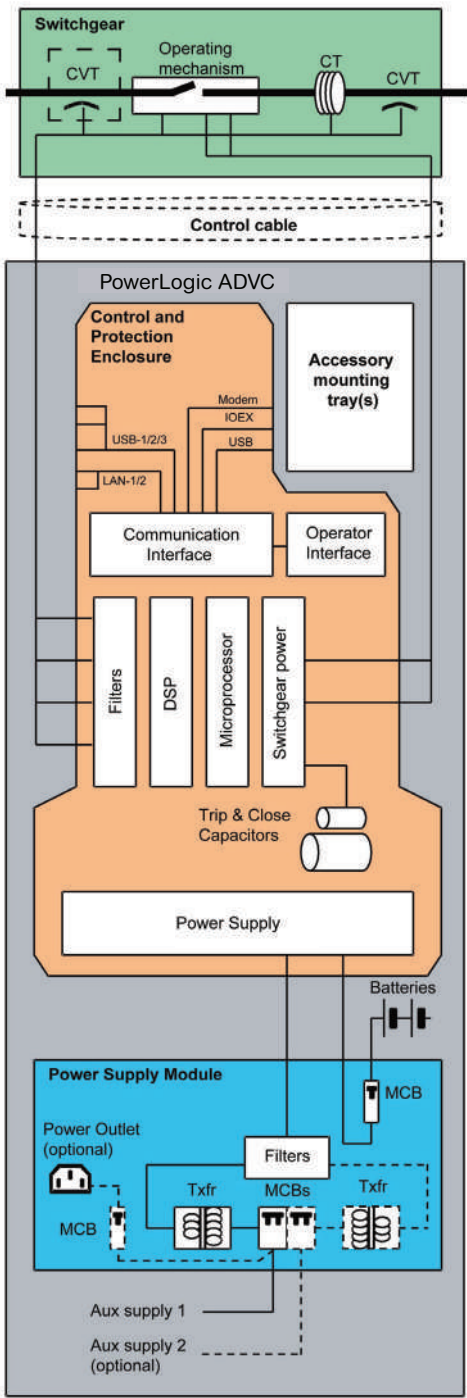
PowerLogic ADVC block diagram
