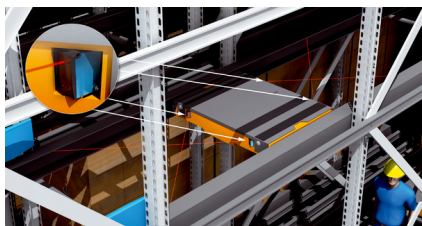
Collision avoidance in shuttle warehouse systems
